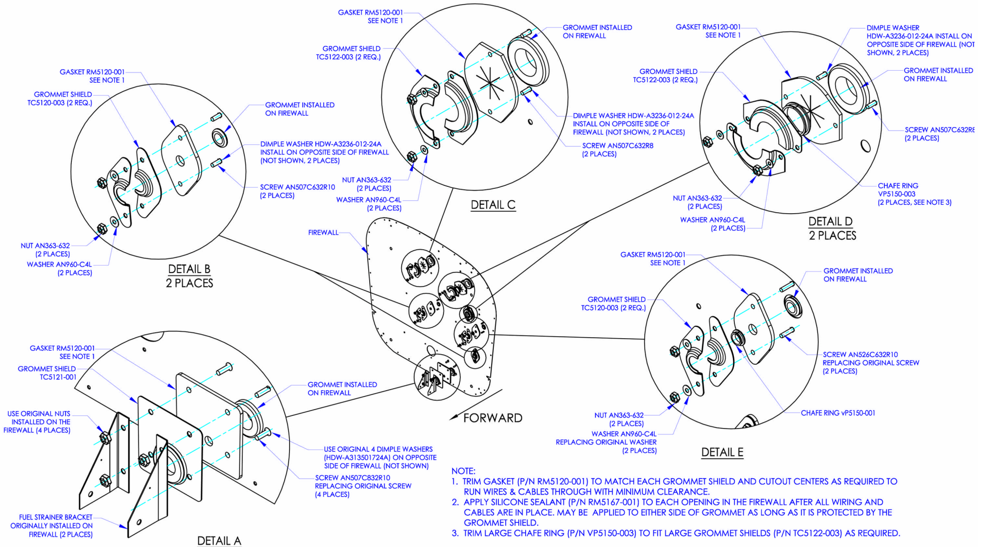
Figure 1: Installation of Firewall Grommet Shields
