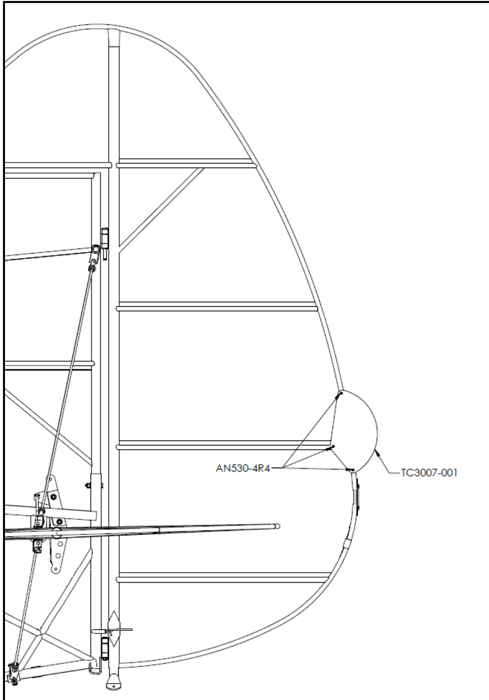
FIGURE 1 – Trim Tab Placement
