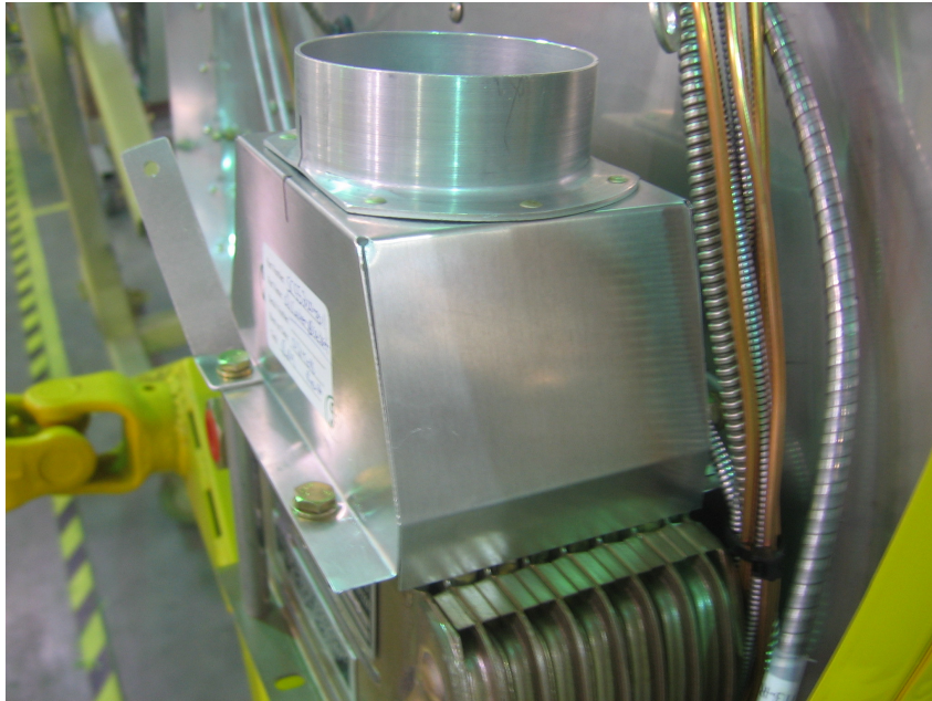
FIGURE 2 - INSTALLATION OF NEW OIL COOLER BRACKET ASSEMBLY
