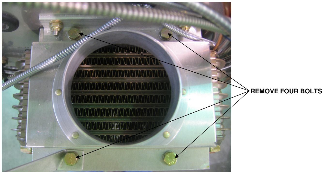
FIGURE 1 - REMOVAL OF TOP OIL COOLER BRACKET ASSEMBLY
