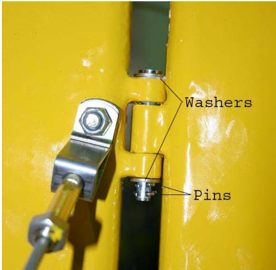
Figure 1 – Rudder Hinge Pin
