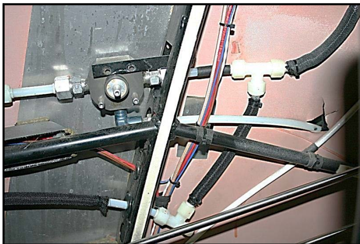
FIGURE 16 – Nylon Tubing Installation
