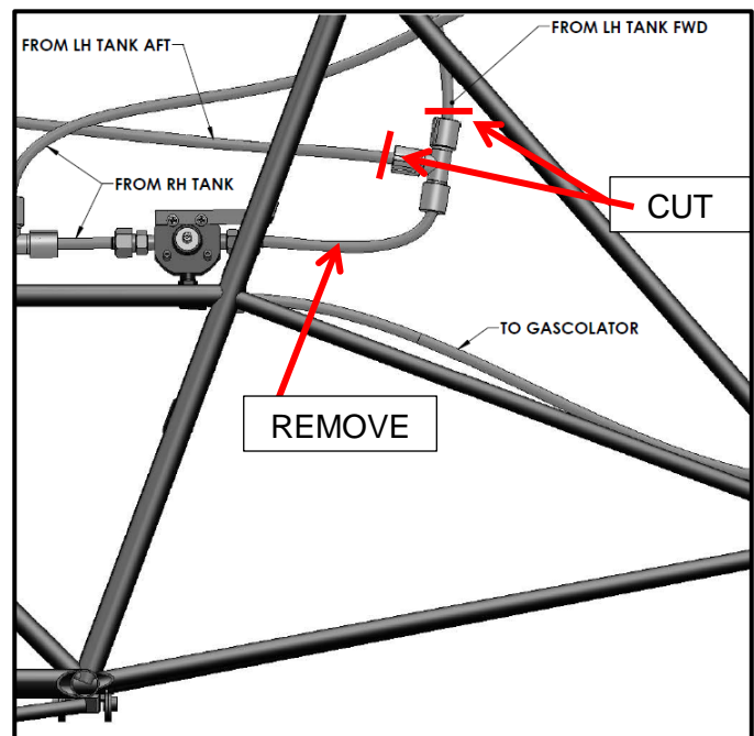
FIGURE 5B – Alternate Fuel Routing
