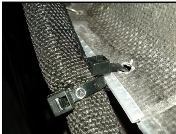
FIGURE 34 – Secure Round-It Protective Wrap using Cable Tie Chain
