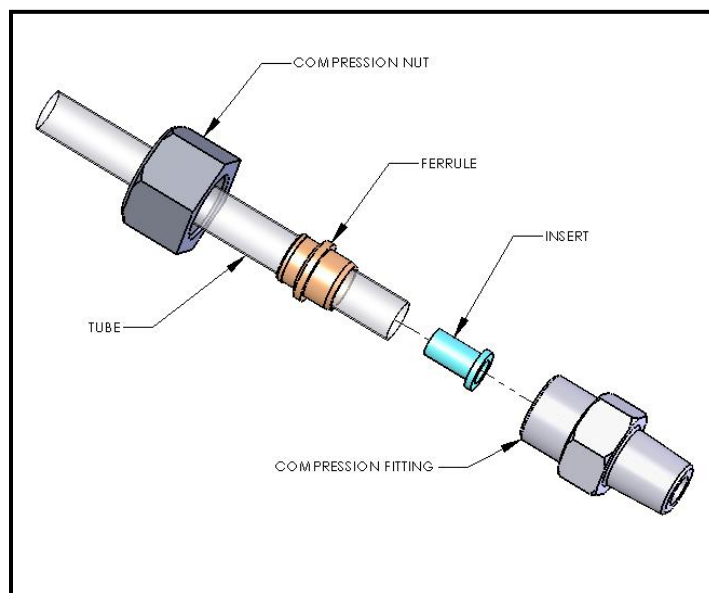
FIGURE 35 – Compression Fitting Assembly
