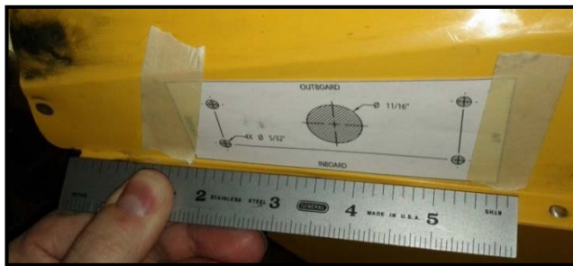
FIGURE 18 – Drill Jig Placement
