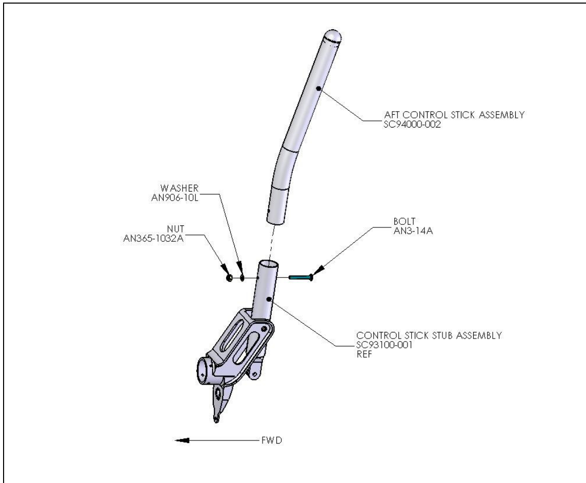
Figure 1– Aft Control Stick
