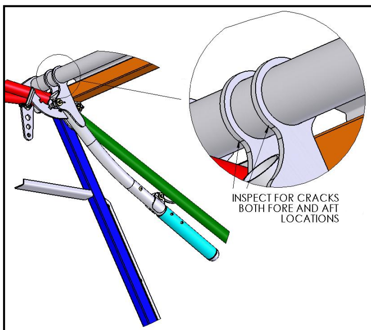
Figure 1 – Inspection Location
