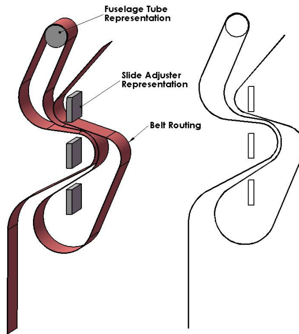
Figure 2 - Side View of Strap Routing
