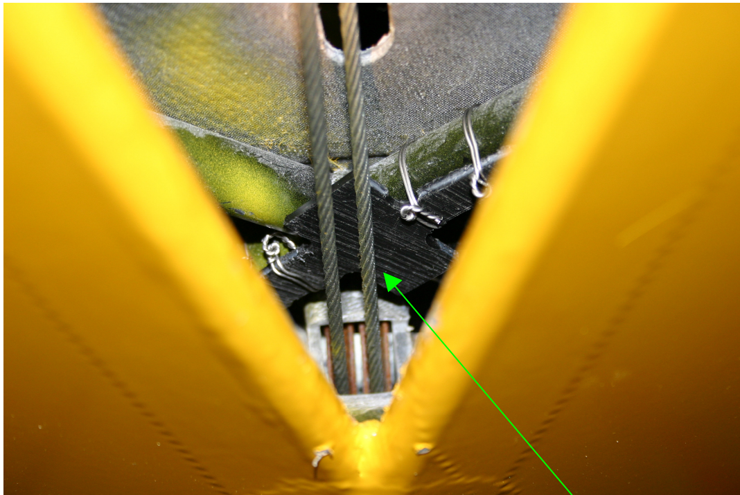
Additional cable rub strip
