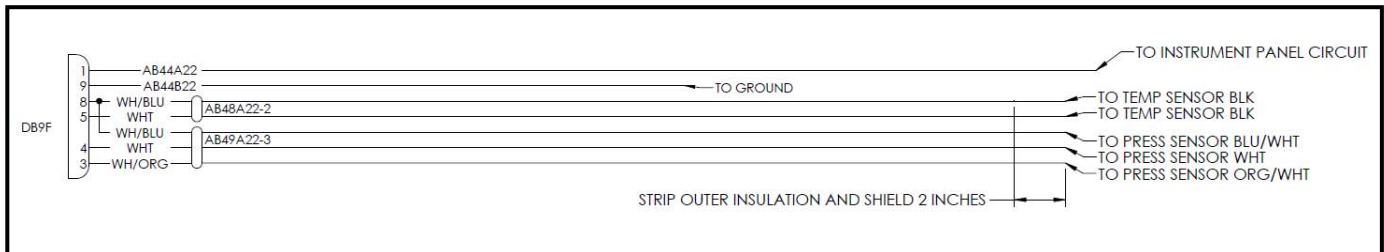
FIGURE 11 – Electronic Gauge Harness (FOR REFERENCE ONLY)
