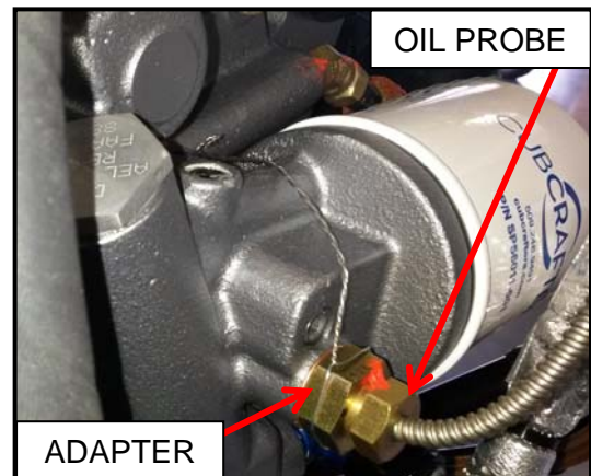
FIGURE 3 - Removal of Existing Port Plug, Bourbon Tube Probe (and Adapter if applicable)
