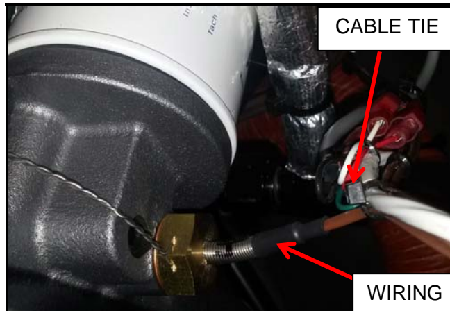
FIGURE 2 – Probe Wiring
