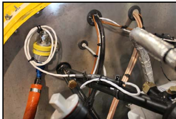
FIGURE 12 – Wire Routing to Sensor (Trim SENSOR wire as needed)
