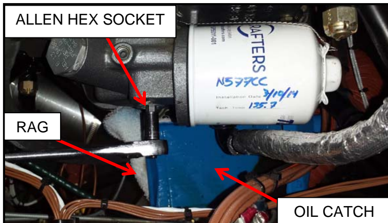
FIGURE 3 - Removal of Existing Port Plug, Bourbon Tube Probe (and Adapter if applicable)
